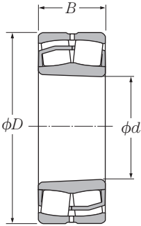
圆锥孔 (EA型)
