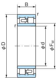
NN 圆柱孔
