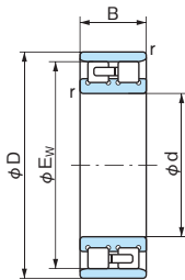
NN 圆柱孔
