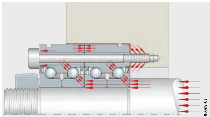
ZKLF Figure 35 Static axial load in the direction of the screw connections
