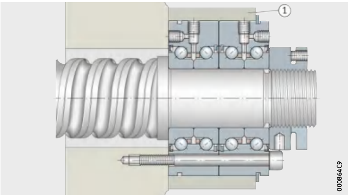
Figure 7 Matched pair, screw mounted on face of adjacent construction, preloaded by locknut AM
