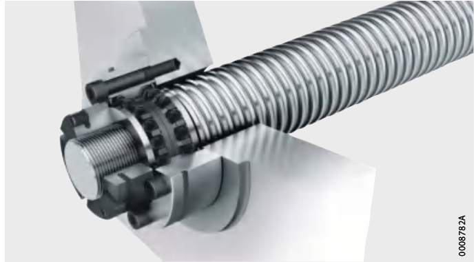
Figure 11 Hybrid axial angular contact ball bearing ZKLF...-HC
