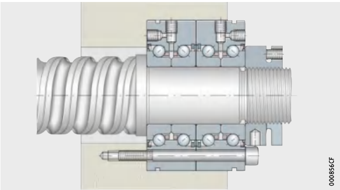
Figure 6 Matched pair, outer ring screw mounted in bore, preloaded by locknut AM
