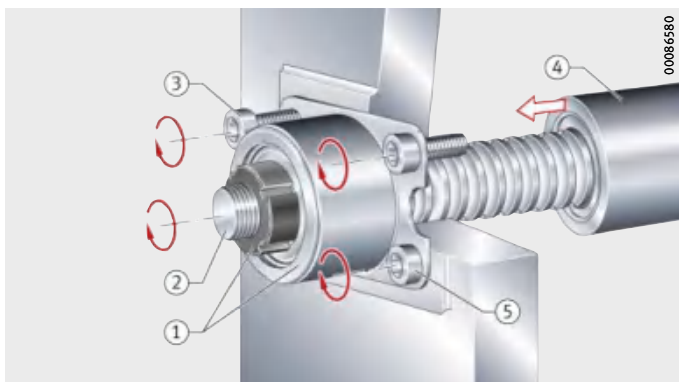
Figure 57 Mounting of bearing unit ZKLK
