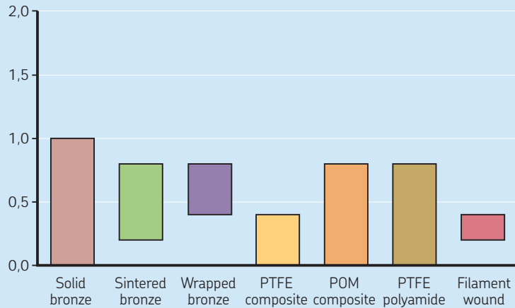
Shaft surface roughness R_a , mm
