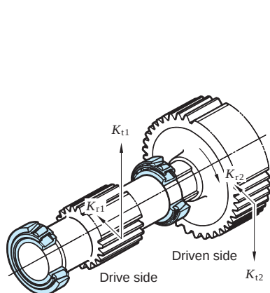
Fig. 5-7 Load on spur gears
