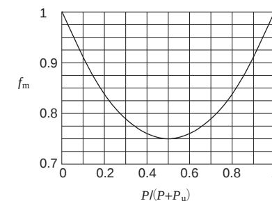
Fig. 5-12 Coefficient f_m
