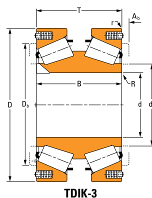
轴承尺寸 额定载荷 100 万转 9000 万转 静态 轴向 内径 外径 外圈宽度 内圈宽度 动态径向 动态轴向 动态径向 K 系数 d D T B C 1(2) e Y C a90 C 90(2) C a0 mm in. mm in. mm in. mm in. kN lbf kN lbf kN lbf kN lbf 305.000 12.0079 559.867 22.0420 176.352 6.9430 273.050 10.7500 2690 605000 0.87 0.68 594 134000 698 157000 0.67 6130 1380000 305.034 12.0092 499.948 19.6830 200.025 7.8750 200.025 7.8750 2370 532000 0.87 0.68 522 117000 613 138000 0.67 6410 1440000 305.034 12.0092 499.948 19.6830 200.025 7.8750 200.025 7.8750 2370 532000 0.87 0.68 522 117000 613 138000 0.67 6410 1440000 305.054 12.0100 499.948 19.6830 200.025 7.8750 200.025 7.8750 2370 532000 0.87 0.68 522 117000 613 138000 0.67 6410 1440000 305.054 12.0100 499.948 19.6830 200.025 7.8750 200.025 7.8750 2330 523000 1.17 0.51 695 156000 603 136000 0.50 6440 1450000 305.034 12.0092 529.500 20.8646 200.000 7.8740 200.000 7.8740 2370 532000 0.98 0.57 522 117000 613 138000 0.67 6410 1440000 330 12.9921 520 20.4724 180 7.0866 180 7.0866 2870 644000 0.87 0.68 633 142000 743 167000 0.67 6830 1540000 340 13.3858 460 18.1102 160 6.2992 160 6.2992 1430 322000 0.71 0.84 260 58500 371 83500 0.82 4020 905000 342.900 13.5000 482.600 19.0000 131.765 5.1876 127.000 5.0000 1530 345000 0.42 1.42 165 37100 398 89500 1.39 2190 493000 355.600 14.0000 533.400 21.0000 200.025 7.8750 200.025 7.8750 3470 781000 0.67 0.89 597 134000 901 203000 0.87 7190 1620000 360 14.1732 480 18.8976 160 6.2992 160 6.2992 1760 396000 0.47 1.27 213 47800 457 103000 1.24 3050 686000 365.600 14.3937 514.350 20.2500 140.000 5.5118 140.000 5.5118 1750 394000 0.74 0.81 330 74300 455 102000 0.79 4800 1080000 368.300 14.5000 596.900 23.5000 165.100 6.5000 158.750 6.2500 3090 694000 0.41 1.44 326 73400 801 180000 1.41 3650 821000 374.650 14.7500 499.745 19.6750 130.175 5.1250 120.650 4.7500 1860 417000 0.47 1.27 224 50300 481 108000 1.24 3020 679000 380 14.9606 548 21.5748 180 7.0866 180 7.0866 2510 563000 0.78 0.77 499 112000 650 146000 0.75 7550 1700000
