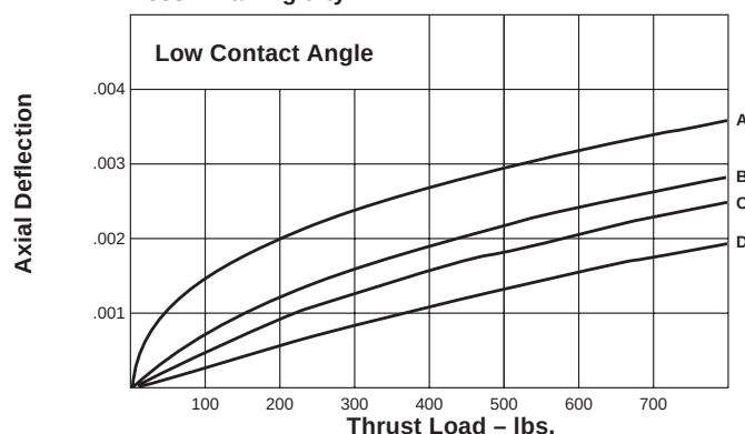
A No Preload B Light Preload 40lbs. C Medium Preload 125lbs. D Heavy Preload 250lbs.
