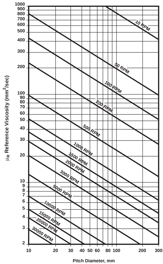
Figure 1 – Determining the Reference Viscosity
