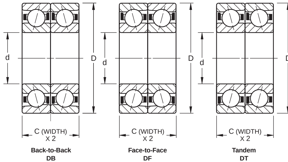
WI Type Duplex Mounting Arrangements
