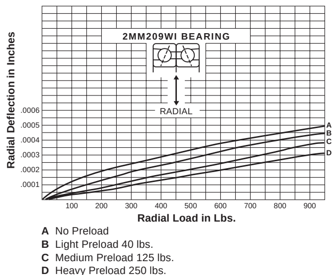
Figure 11 – Radial Deflection Curves
