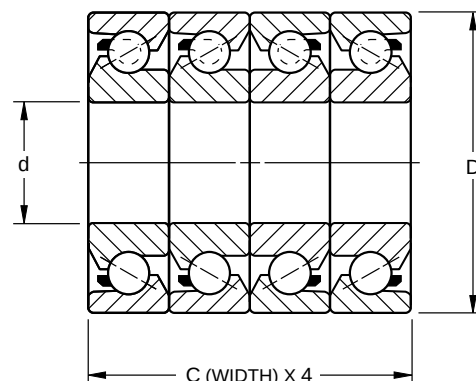
Quadruplex Mounting
