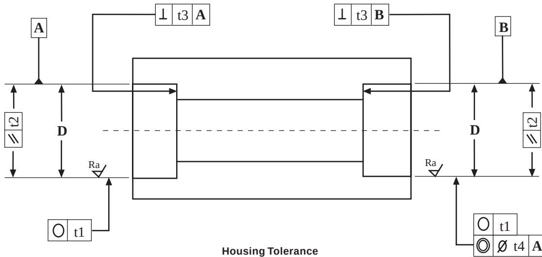
Housing Tolerance
