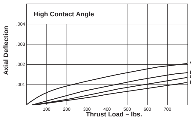
A No Preload B Light Preload 40lbs. C Medium Preload 125lbs. D Heavy Preload 250lbs.
