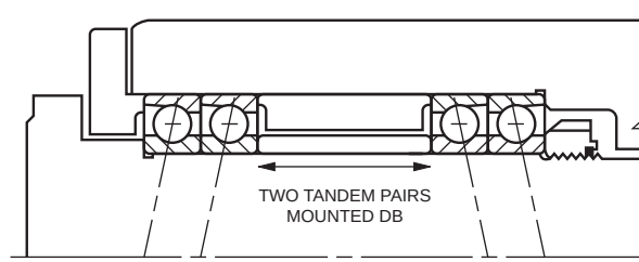
Figure 9 – DT-DB Mounting, Fixed
