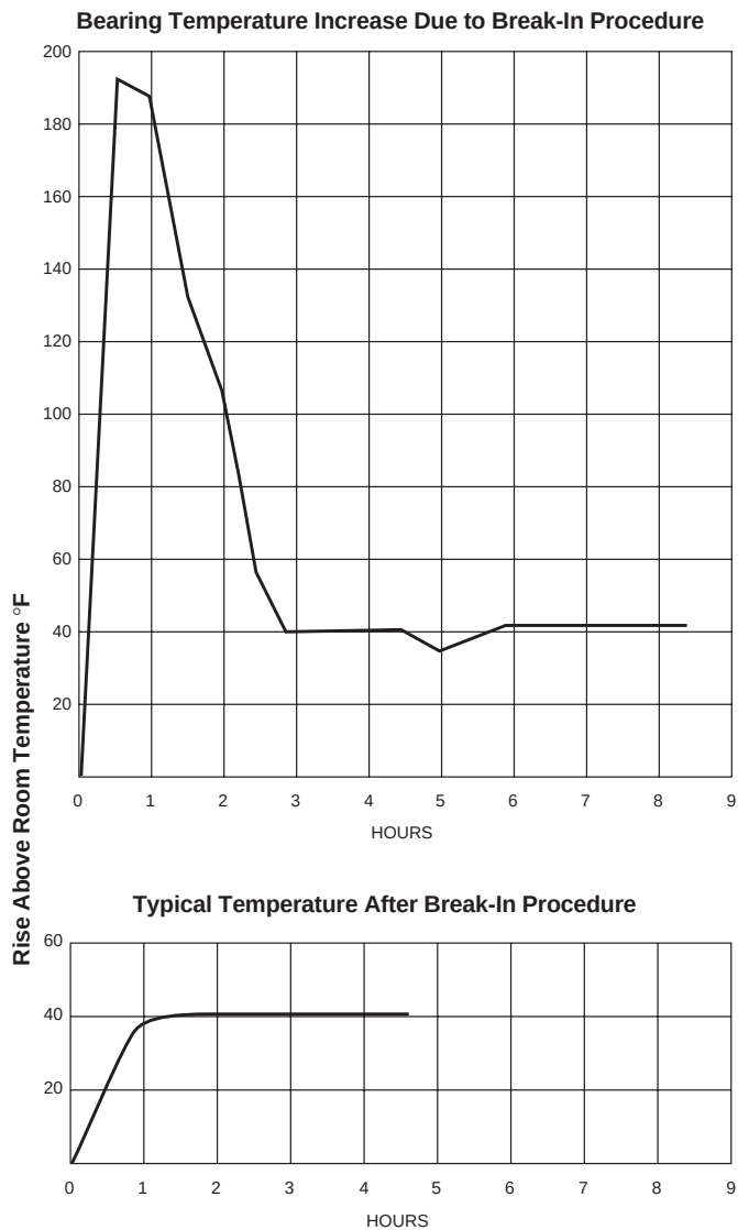
Figure 16 – Temperature vs Time
