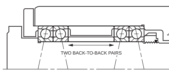
Figure 7 – DB-DB Mounting, Fixed (Not Recommended)
