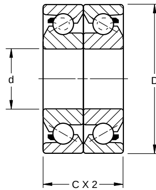
Duplex Mounting
