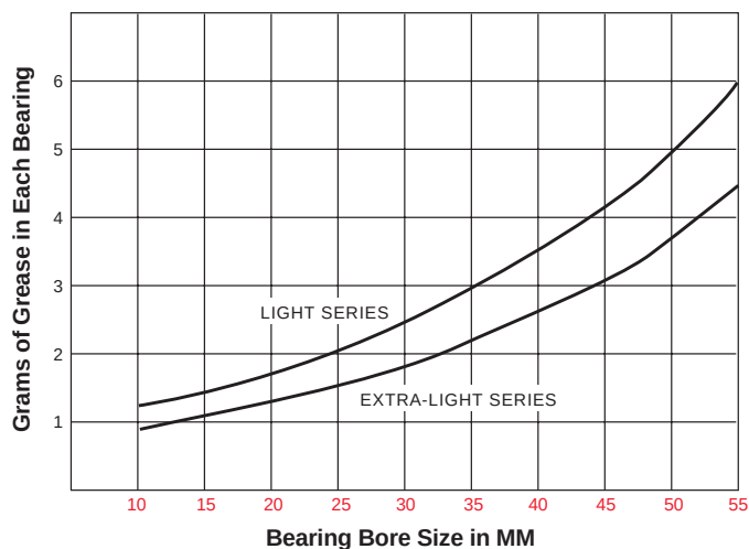
Figure 17 – Grease Quantity Chart
