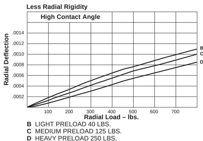
Figure 14 – Radial Deflections
