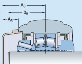
SYNT series
