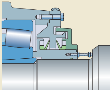
Labyrinth seal with two V-ring seals
