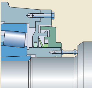
Labyrinth seal with one V-ring seal
