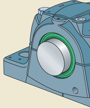
New position of grease escape hole
