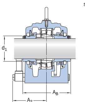
Housing for through shaft
