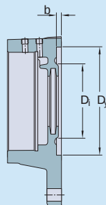
Centring recess on FNL housings
