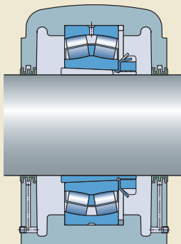
Plain shaft with bearing on an adapter sleeve
