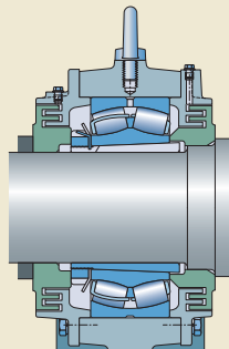
Stepped shaft with bearing on an adapter sleeve, designation suffix C
