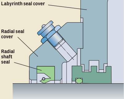
Multi-seal
