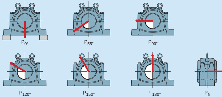
Safe loads for large SNL plummer block housings made of grey cast iron
