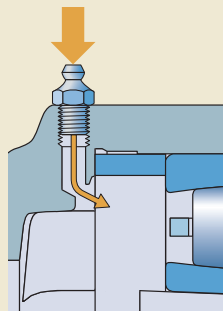
Grease guiding system
