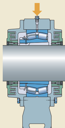
Grease fitting in THD housing
