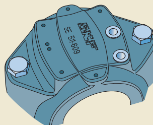
Improved position for relubrication
