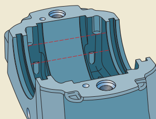
Grease level markings
