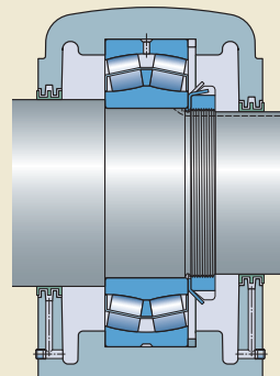
Stepped shaft with bearing on a cylindrical seat
