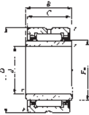
NA49...U NA69...U( d \leq 30 )
