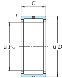
NK ( u F_w \geq 12 ), NKS, RNA48, RNA49, RNA69 ( u F_w \leq 35 )
