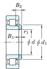
Thrust collar
