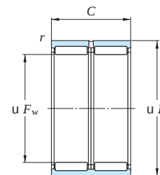
RNA69 ( u F_w \geq 40 )
