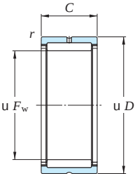
NK ( u F_w \geq 12 ), NKS, RNA48, RNA49, RNA69 ( u F_w \leq 35 )
