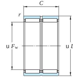
RNA69 ( u F_w \geq 40 )
