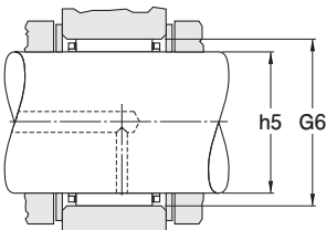
raceway surfaces to be 58 HRC or equivalent
