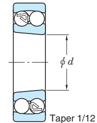
Tapered bore Taper 1/12
