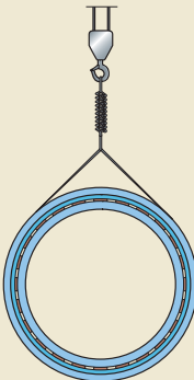
Mounting a heated large bearing
